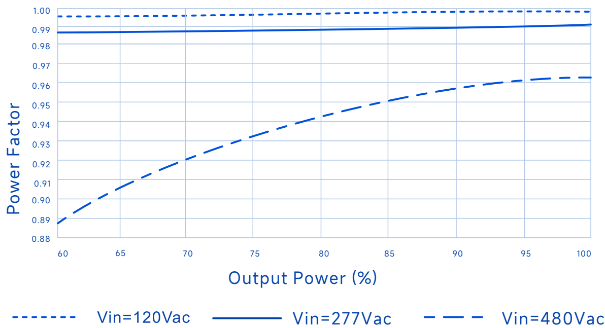
Power Factor Vs. Output Power
